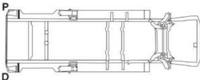
UNDERBODY VIEW
